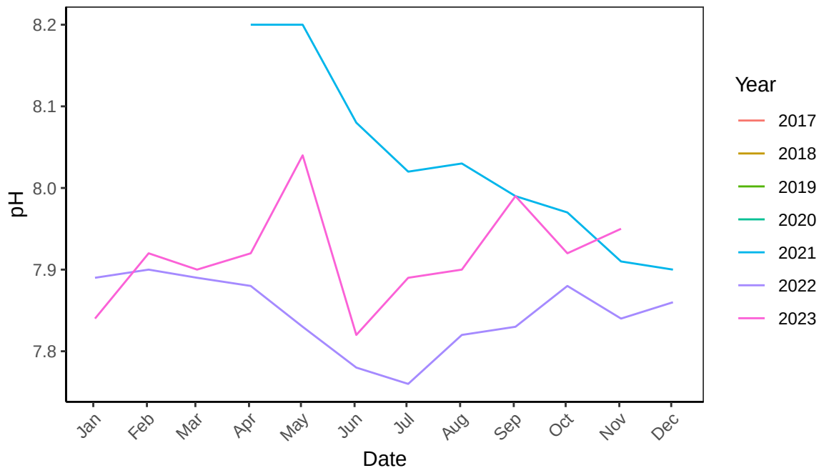
B2 Raceway 2 pH Monthly Statistics
